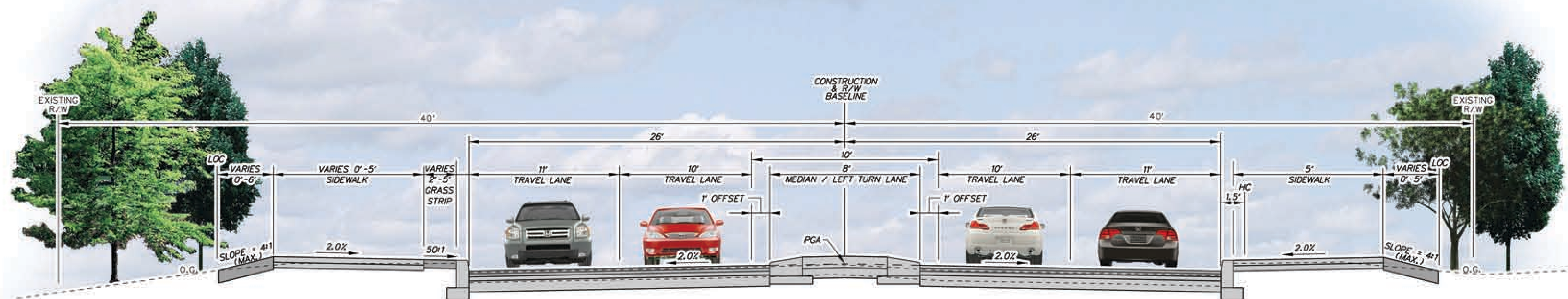
WILSON ROAD - TYPICAL SECTION
