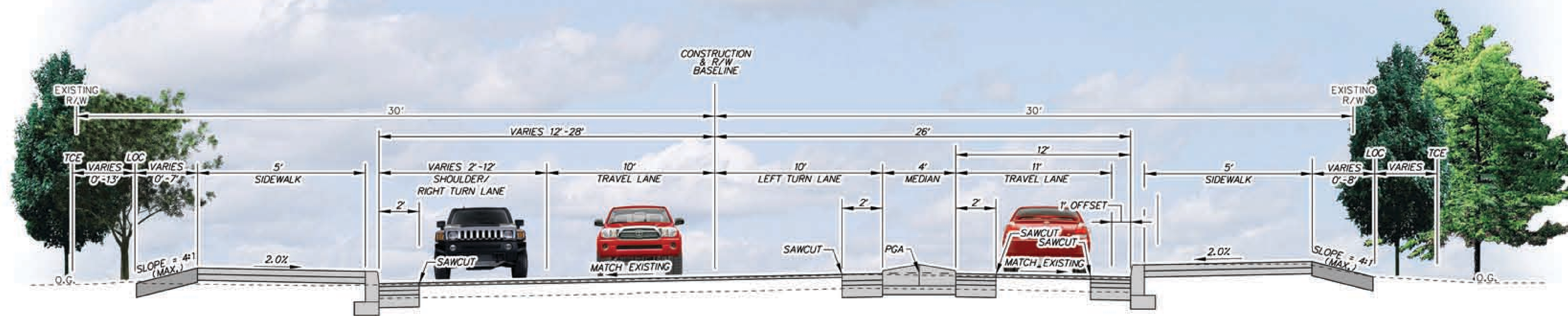
FOULK ROAD - TYPICAL SECTION
